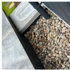
Paraprt wall drainage chanel blocked with pebbles Also, no secondsry drainage chanel. 25/05/2022 11:13 (BST)
